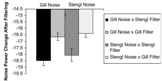
Figure 5 Mean ( \pm SE) change in power (in arbitrary dB units) in the noise spectra from the Gill and Stengl locations after filtering with the Stengl and Gill filters. Larger negative numbers indicate less noise remaining thus indicating that more noise was rejected by the filter. Filtering is independent of absolute noise level.
